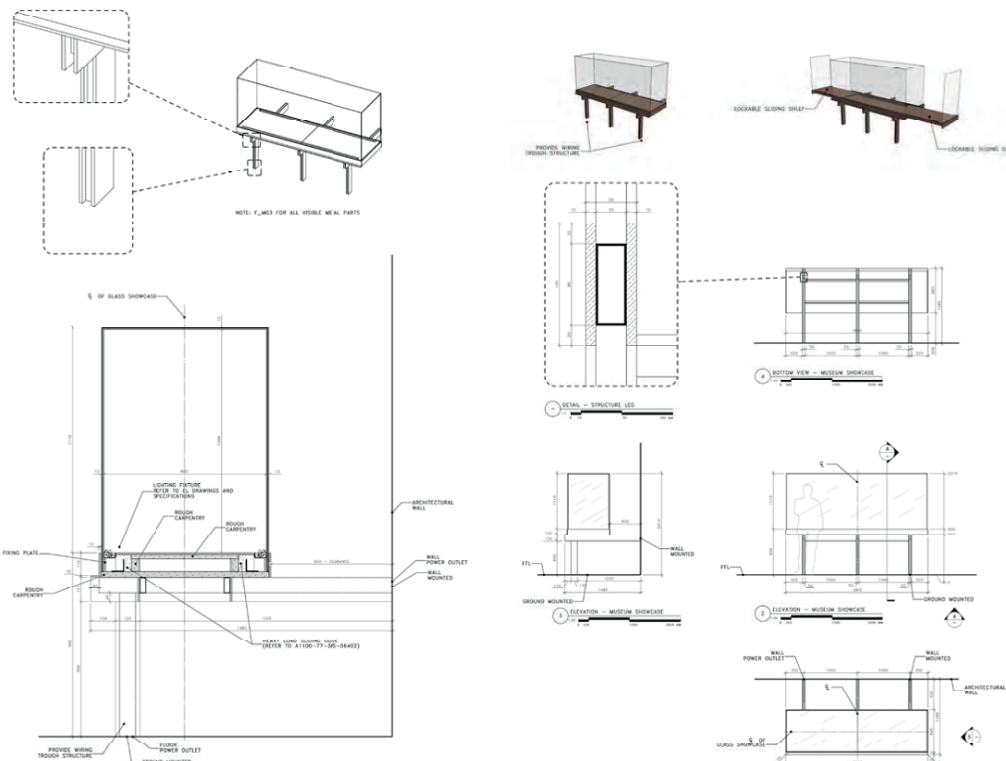
Museum Gallery partial elevation
