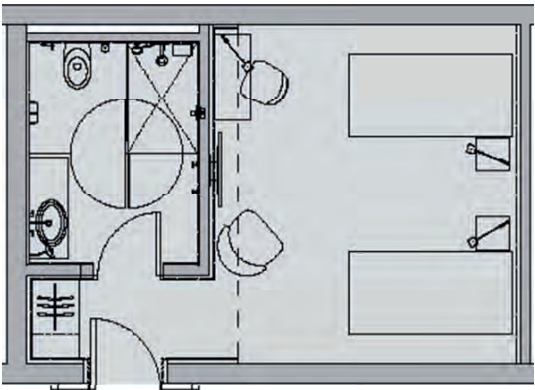
Treatment room floor plan
